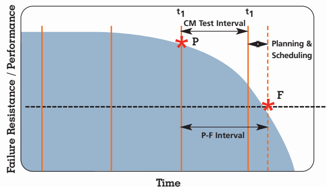
Figure 2: Sizing the CM Test Interval
