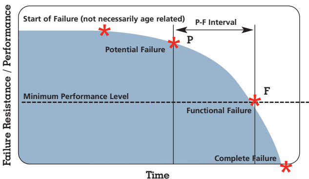
Figure 1: The P-F Curve
